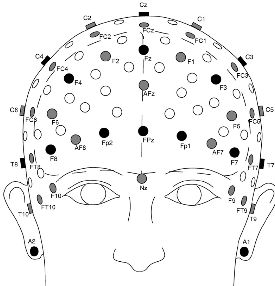
Anterior view of 10-10 system electrode positions and labels Oostenveld and Praamstra (2000).
