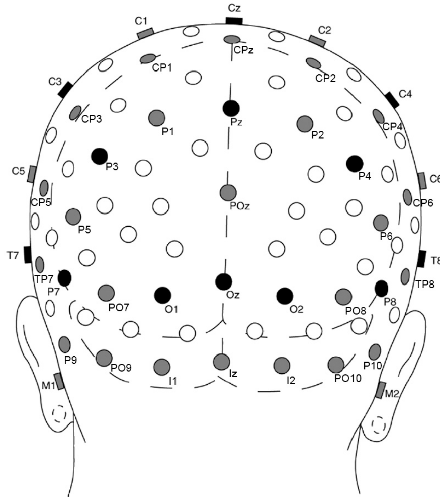
Posterior view of 10-10 system electrode positions and labels Oostenveld and Praamstra (2000).
