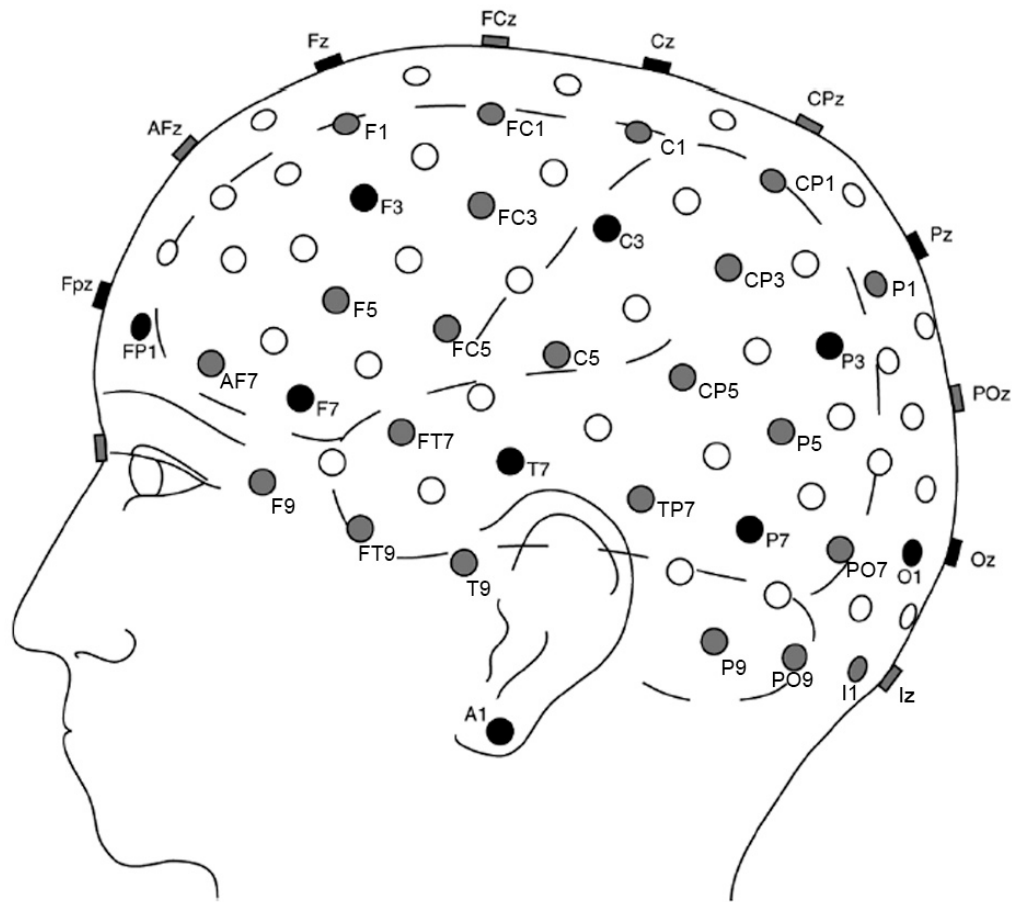
Lateral view of 10-10 system electrode positions and labels Oostenveld and Praamstra (2000).
